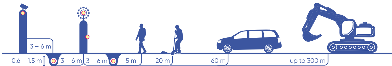
Maximum distance from fiber-optic cable for registration and classification of vibroacoustic influences
